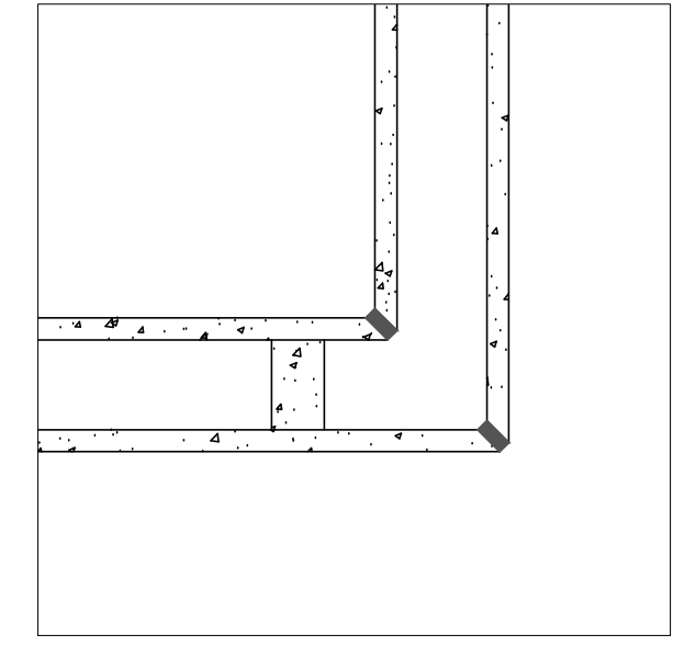
CORNER DETAIL (TYP)
